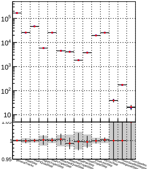
Number —●— DQM_TT__mkFit-DQM_mod
