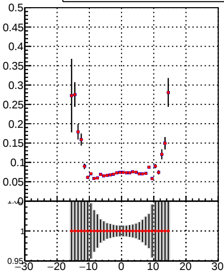
—●— DQM_TT_mkFit-DQM_orig —●— DQM_TT_mkFit-DQM_mod
