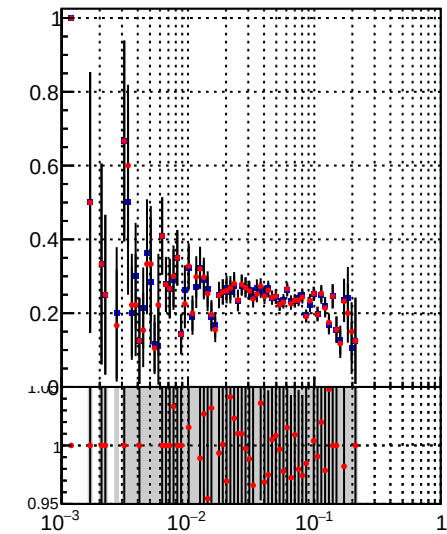
■ DQM_TT_mkFit-DQM_orig ● DQM_TT_mkFit-DQM_mod
