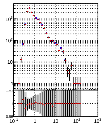
—●— DQM_TT_mkFit-DQM_orig —●— DQM_TT_mkFit-DQM_mod
