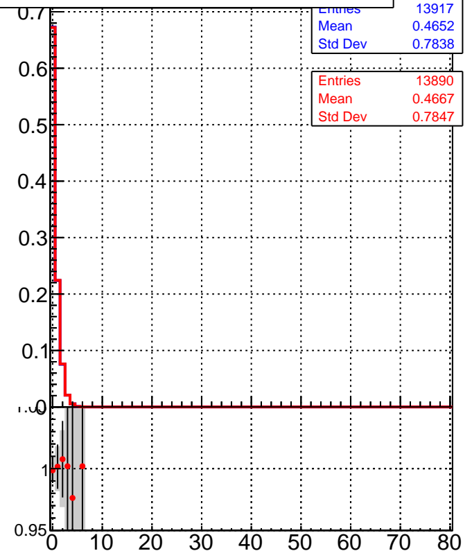
■ DQM_TT_mkFit-DQM_orig ● DQM_TT_mkFit-DQM_mod
