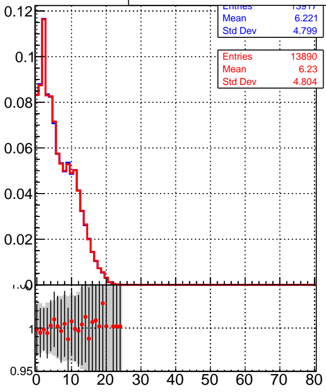
■ DQM_TT_mkFit-DQM_orig ● DQM_TT_mkFit-DQM_mod
