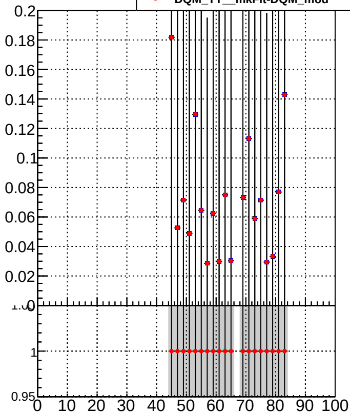
—■ DQM_TT_mkFit-DQM_orig —● DQM_TT_mkFit-DQM_mod
