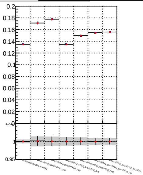
Fake rate vs. —●— DQM_TT mkFit-DQM_orig —●— DQM_TT mkFit-DQM_mod
