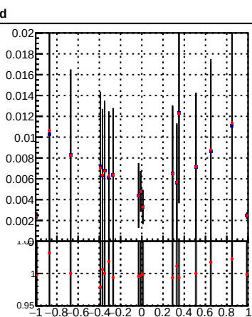
Duplicates Rate vs Dz(PV)
