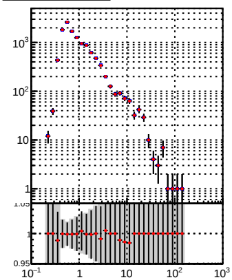
N of reco track vs \eta DQM_TT_mkFit-DQM_orig DQM_TT_mkFit-DQM_mod
