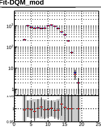
DQM_TT_mkFit-DQM_orig DQM_TT_mkFit-DQM_mod
