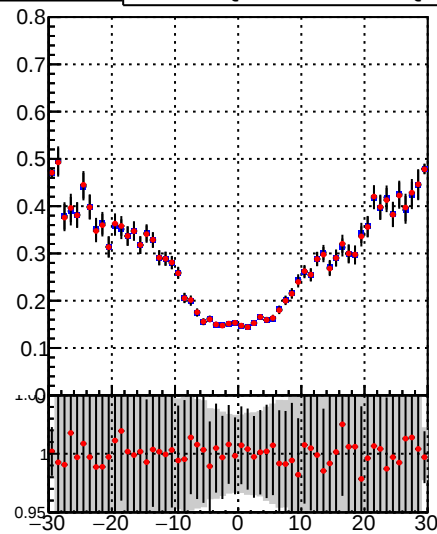
—●— DQM_TT_mkFit-DQM_orig —●— DQM_TT_mkFit-DQM_mod
