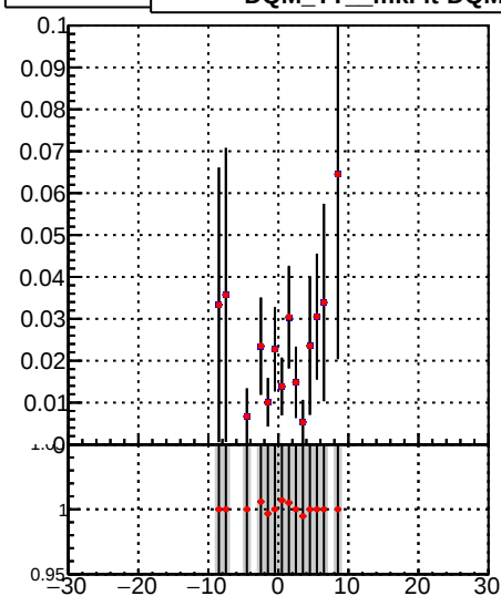
Fake rate vs verpos
