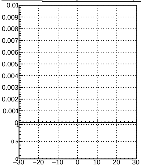
Fake rate vs v DQM_TT_mkFit-DQM_orig DQM_TT_mkFit-DQM_mod
