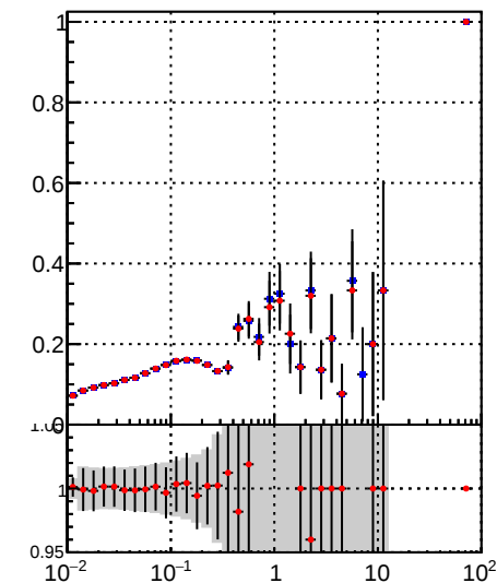
—•— DQM_TT_mkFit-DQM_orig —•— DQM_TT_mkFit-DQM_mod
