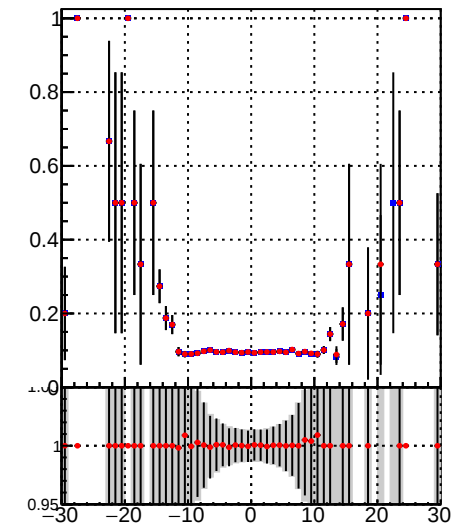
—•— DQM_TT_mkFit-DQM_orig —•— DQM_TT_mkFit-DQM_mod
