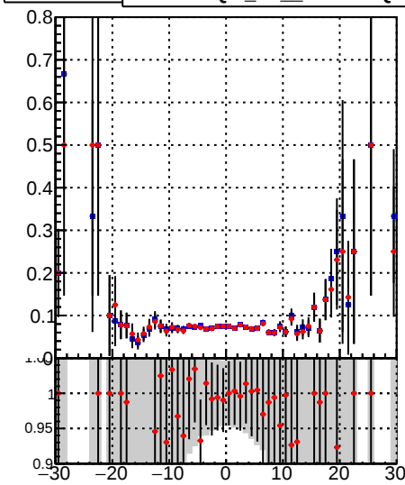
—•— DQM_TT_mkFit-DQM_orig —•— DQM_TT_mkFit-DQM_mod
