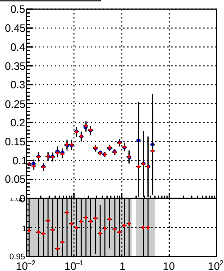
—•— DQM_TT_mkFit-DQM_orig —•— DQM_TT_mkFit-DQM_mod
