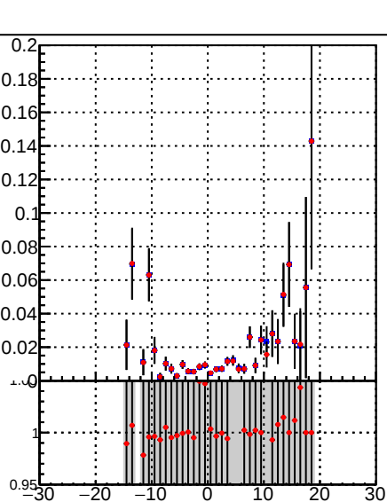
—•— DQM_TT_mkFit-DQM_orig —•— DQM_TT_mkFit-DQM_mod
