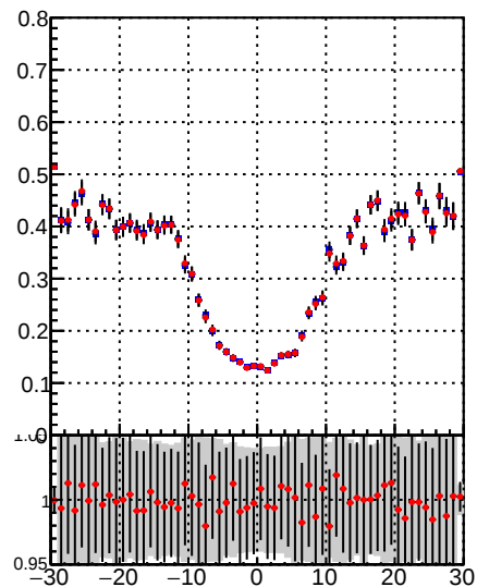
—●— DQM_TT_mkFit-DQM_orig —●— DQM_TT_mkFit-DQM_mod
