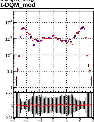
N of associated (recoToSim) tracks vs phi
