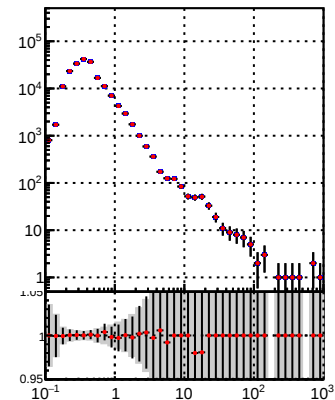
—•— DQM_TT_mkFit-DQM_orig —•— DQM_TT_mkFit-DQM_mod
