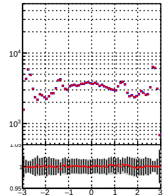
—•— DQM_TT_mkFit-DQM_orig —•— DQM_TT_mkFit-DQM_mod
