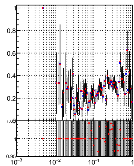
—●— DQM_TT_mkFit-DQM_orig —●— DQM_TT_mkFit-DQM_mod
