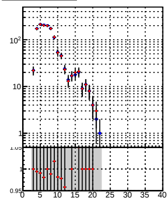
N of reco track vs hit DQM_TT_mkFit-DQM_orig DQM_TT_mkFit-DQM_mod
