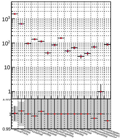
Number —●— DQM_TT__mkFit-DQM_mod
