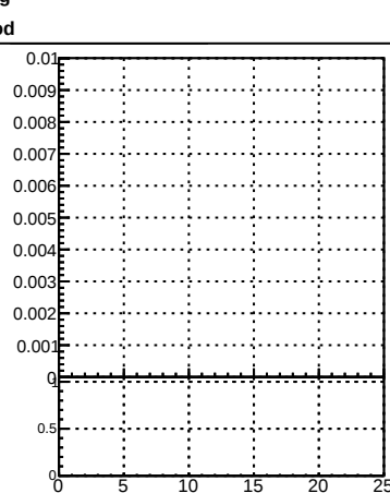
Duplicates Rate vs hit
