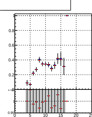
Pileup rate vs hit
