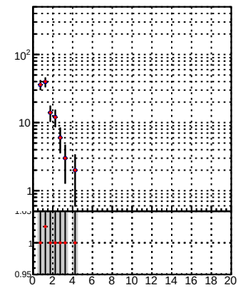
N of associated (recoToSim) tracks vs. s
