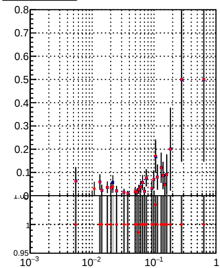
Fake rate vs \epsilon Legend: DQM_TT_mkFit-DQM_orig (blue line with dots) DQM_TT_mkFit-DQM_mod (red line with dots)
