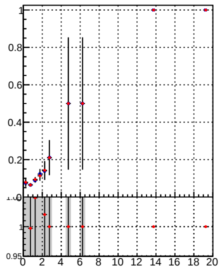
Fake rate vs. —•— DQM_TT_mkFit-DQM_orig —•— DQM_TT_mkFit-DQM_mod
