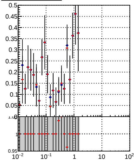
—•— DQM_TT_mkFit-DQM_orig —•— DQM_TT_mkFit-DQM_mod
