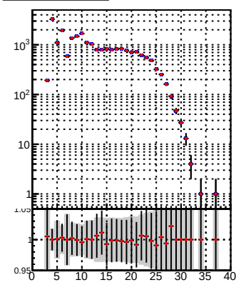
■ DQM_TT_mkFit-DQM_orig — DQM_TT_mkFit-DQM_mod
