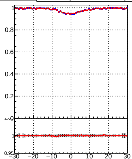
—•— DQM_TT_mkFit-DQM_orig —•— DQM_TT_mkFit-DQM_mod
