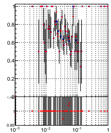
—•— DQM_TT_mkFit-DQM_orig —•— DQM_TT_mkFit-DQM_mod
