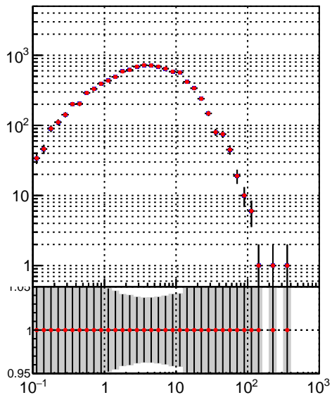
■ DQM_TT_mkFit-DQM_orig ◆ DQM_TT_mkFit-DQM_mod
