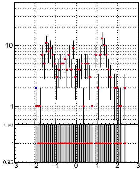
■ DQM_TT_mkFit-DQM_orig ◆ DQM_TT_mkFit-DQM_mod
