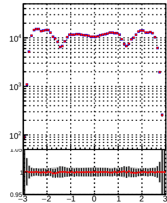
N of reco track vs \eta pT eta Legend: —•— DQM_TT_mkFit-DQM_orig —•— DQM_TT_mkFit-DQM_mod
