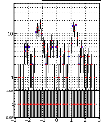
—•— DQM_TT_mkFit-DQM_orig —•— DQM_TT_mkFit-DQM_mod
