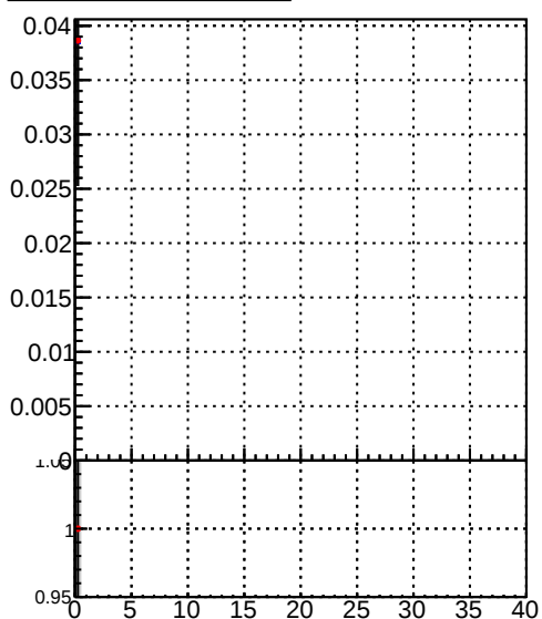
\Delta efficiency vs R (radial)
