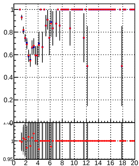
\Delta fake rate vs p_T
