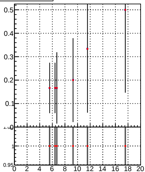
\Delta efficiency vs p_T
