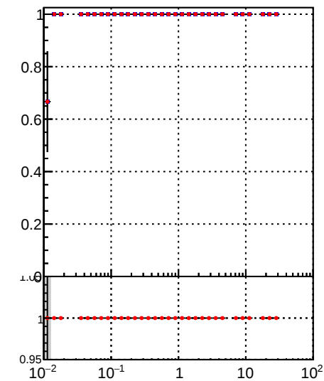
Fake rate vs vertpos Legend: DQM_TT_mkFit-DQM_orig (grey line) DQM_TT_mkFit-DQM_mod (red line)
