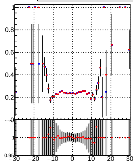
—●— DQM_TT_mkFit-DQM_orig —●— DQM_TT_mkFit-DQM_mod
