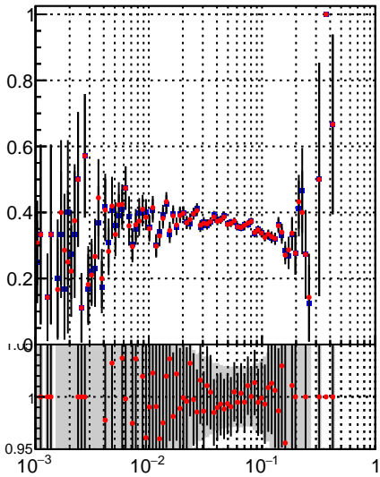
■ DQM_TT_mkFit-DQM_orig ● DQM_TT_mkFit-DQM_mod
