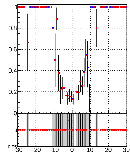
—•— DQM_TT_mkFit-DQM_orig —•— DQM_TT_mkFit-DQM_mod
