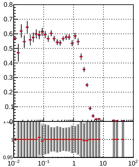
Efficiency vs vert r Legend: — DQM_TT_mkFit-DQM_orig — DQM_TT_mkFit-DQM_mod
