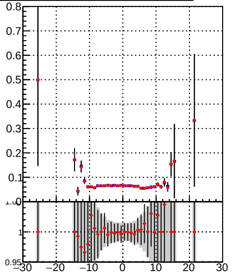
Efficiency vs vert r Legend: — DQM_TT_mkFit-DQM_orig — DQM_TT_mkFit-DQM_mod
