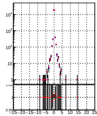
DQM_TT_mkFit-DQM_orig DQM_TT_mkFit-DQM_mod
