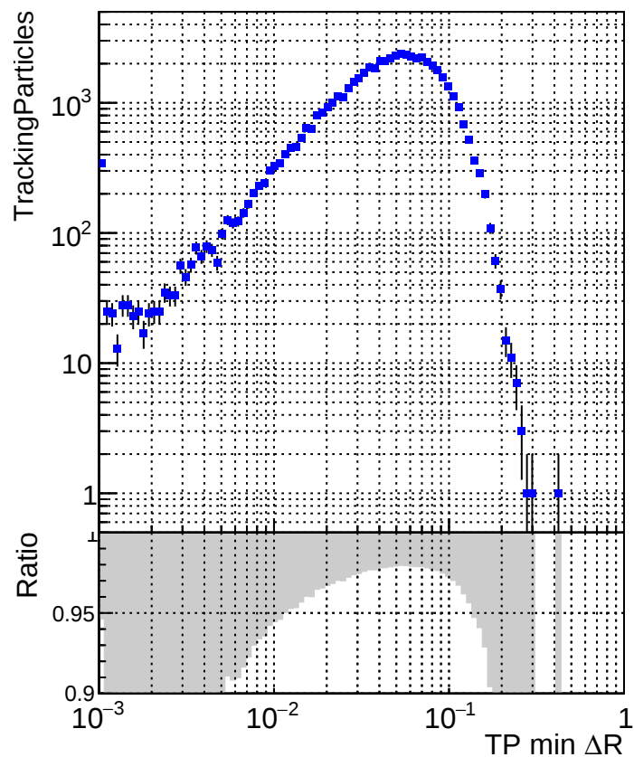
N of simulated tracks vs \Delta R (TP, jet)
