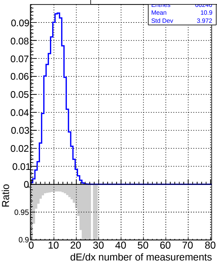
DQM_TT_original
