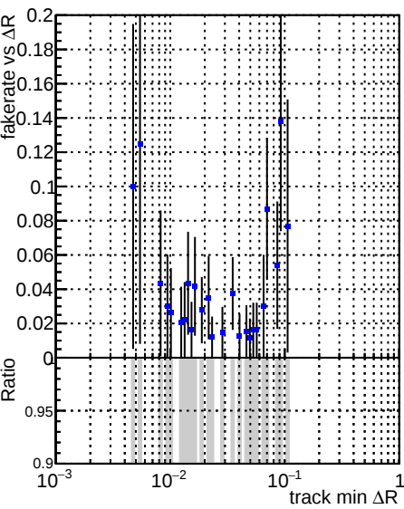
Fake rate vs ΔR(track, jet) DQM_TT_original
