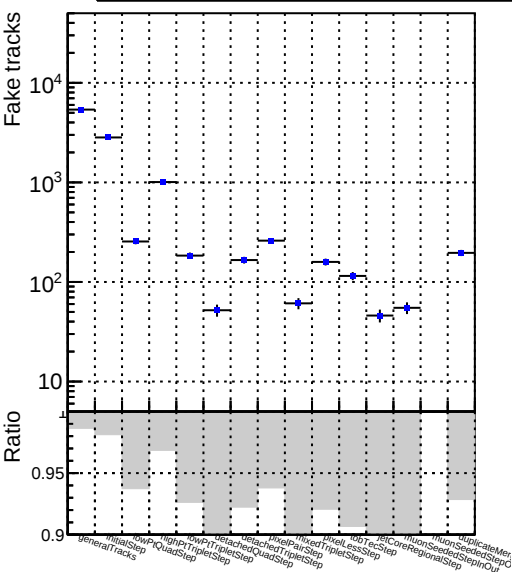
Number DQM_TT__original 1 0 2 0 3 0 4 0 5 0 6 0 7 0 8 0 9 0 10 0 11 0 12 0 13 0 14 0 15 0 16 0 17 0 18 0 19 0 20 0 21 0 22 0 23 0 24 0 25 0 26 0 27 0 28 0 29 0 30 0 31 0 32 0 33 0 34 0 35 0 36 0 37 0 38 0 39 0 40 0 41 0 42 0 43 0 44 0 45 0 46 0 47 0 48 0 49 0 50 0 51 0 52 0 53 0 54 0 55 0 56 0 57 0 58 0 59 0 60 0 61 0 62 0 63 0 64 0 65 0 66 0 67 0 68 0 69 0 70 0 71 0 72 0 73 0 74 0 75 0 76 0 77 0 78 0 79 0 80 0 81 0 82 0 83 0 84 0 85 0 86 0 87 0 88 0 89 0 90 0 91 0 92 0 93 0 94 0 95 0 96 0 97 0 98 0 99 0 100 0 101 0 102 0 103 0 104 0 105 0 106 0 107 0 108 0 109 0 110 0 111 0 112 0 113 0 114 0 115 0 116 0 117 0 118 0 119 0 120 0 121 0 122 0 123 0 124 0 125 0 126 0 127 0 128 0 129 0 130 0 131 0 132 0 133 0 134 0 135 0 136 0 137 0 138 0 139 0 140 0 141 0 142 0 143 0 144 0 145 0 146 0 147 0 148 0 149 0 150 0 151 0 152 0 153 0 154 0 155 0 156 0 157 0 158 0 159 0 160 0 161 0 162 0 163 0 164 0 165 0 166 0 167 0 168 0 169 0 170 0 171 0 172 0 173 0 174 0 175 0 176 0 177 0 178 0 179 0 180 0 181 0
