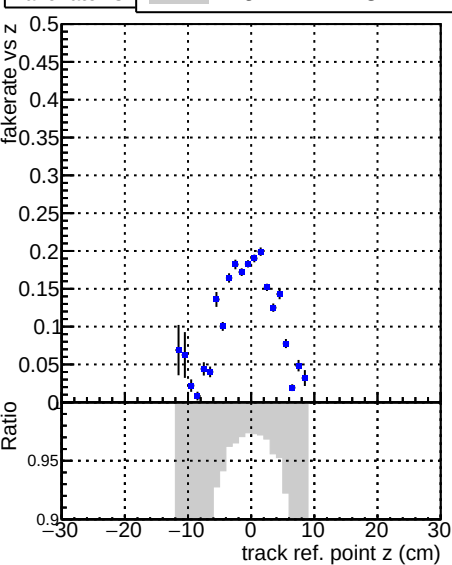
Fake rate vs v DQM_TT__original
