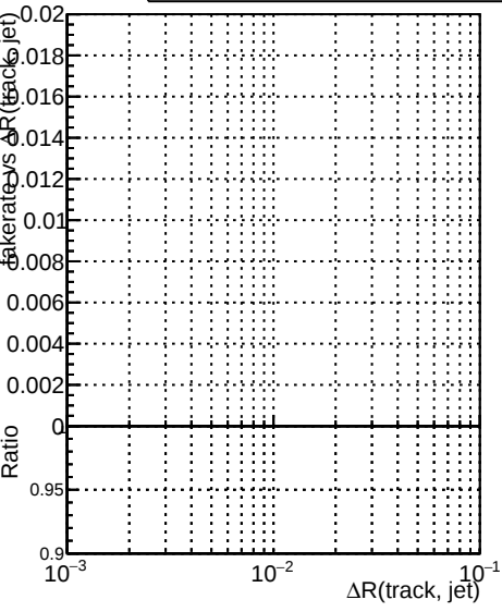
Fake rate vs \Delta R(\text{track, jet}) DQM_TT_original
