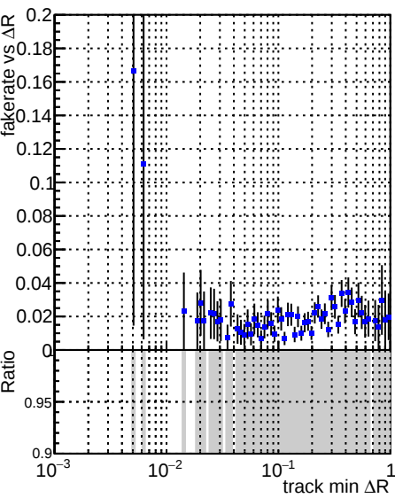
Fake rate vs \Delta R(\text{track, jet}) DQM_TT_original
