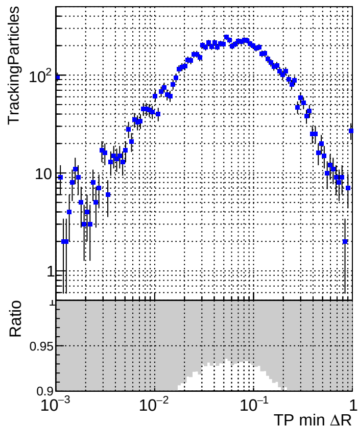
N of simulated tracks vs \Delta R
