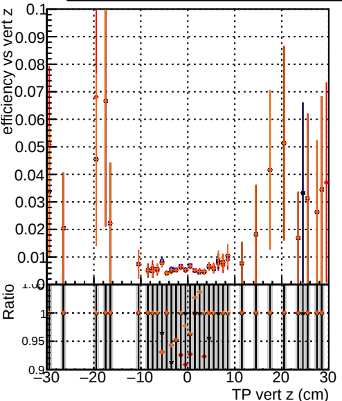
Efficiency vs vertpos DQM_original_step2_ttbar-phase1-newgeom DQM_mkFit_step2_ttbar-phase1-newgeom DQM_angle_step2_ttbar-phase1-newgeom DQM_fast_step2_ttbar-phase1-newgeom
