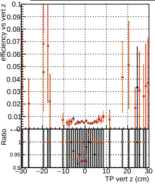
Efficiency vs vert z Legend: DQM_original_step2_ttbar-phase1-newgeom DQM_mkFit_step2_ttbar-phase1-newgeom DQM_angle_step2_ttbar-phase1-newgeom DQM_fast_step2_ttbar-phase1-newgeom
