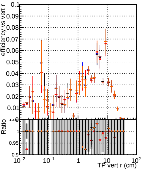
Efficiency vs TP vert r (cm) DQM_original_step2_ttbar-phase1-newgeom DQM_mkFit_step2_ttbar-phase1-newgeom DQM_angle_step2_ttbar-phase1-newgeom DQM_fast_step2_ttbar-phase1-newgeom
